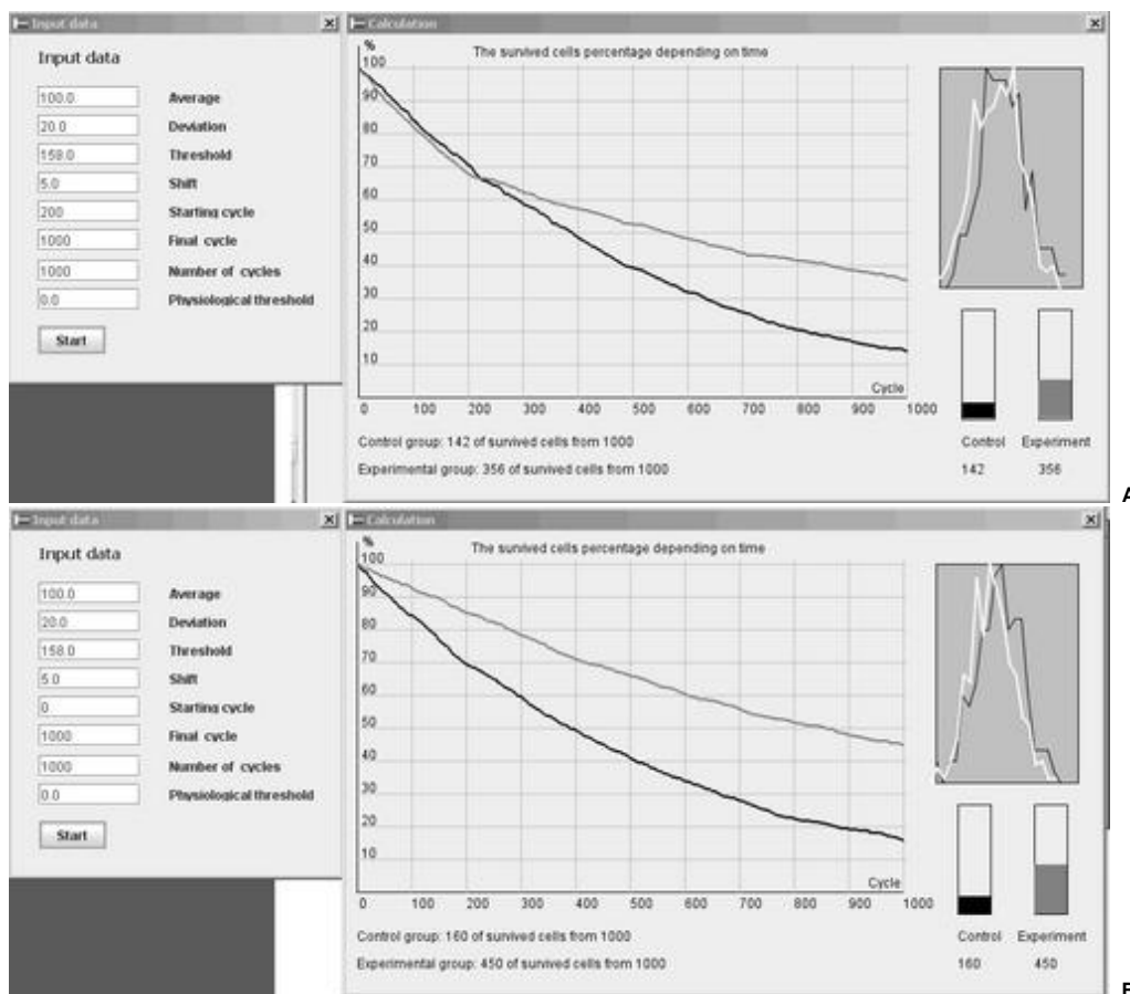
Fig. 2. A screen layout at carrying computer modelling out with using the developed model. A - introduction of the protector from the 200th cycle, B - from a zero cycle.
