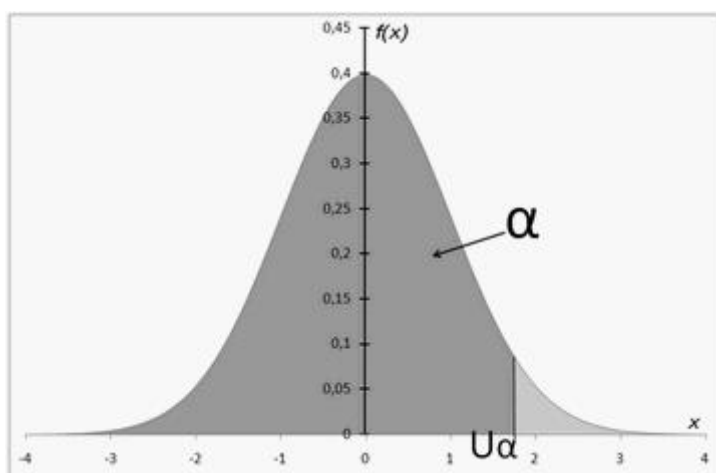
Fig. 1. The normalized curve of normal distribution.
